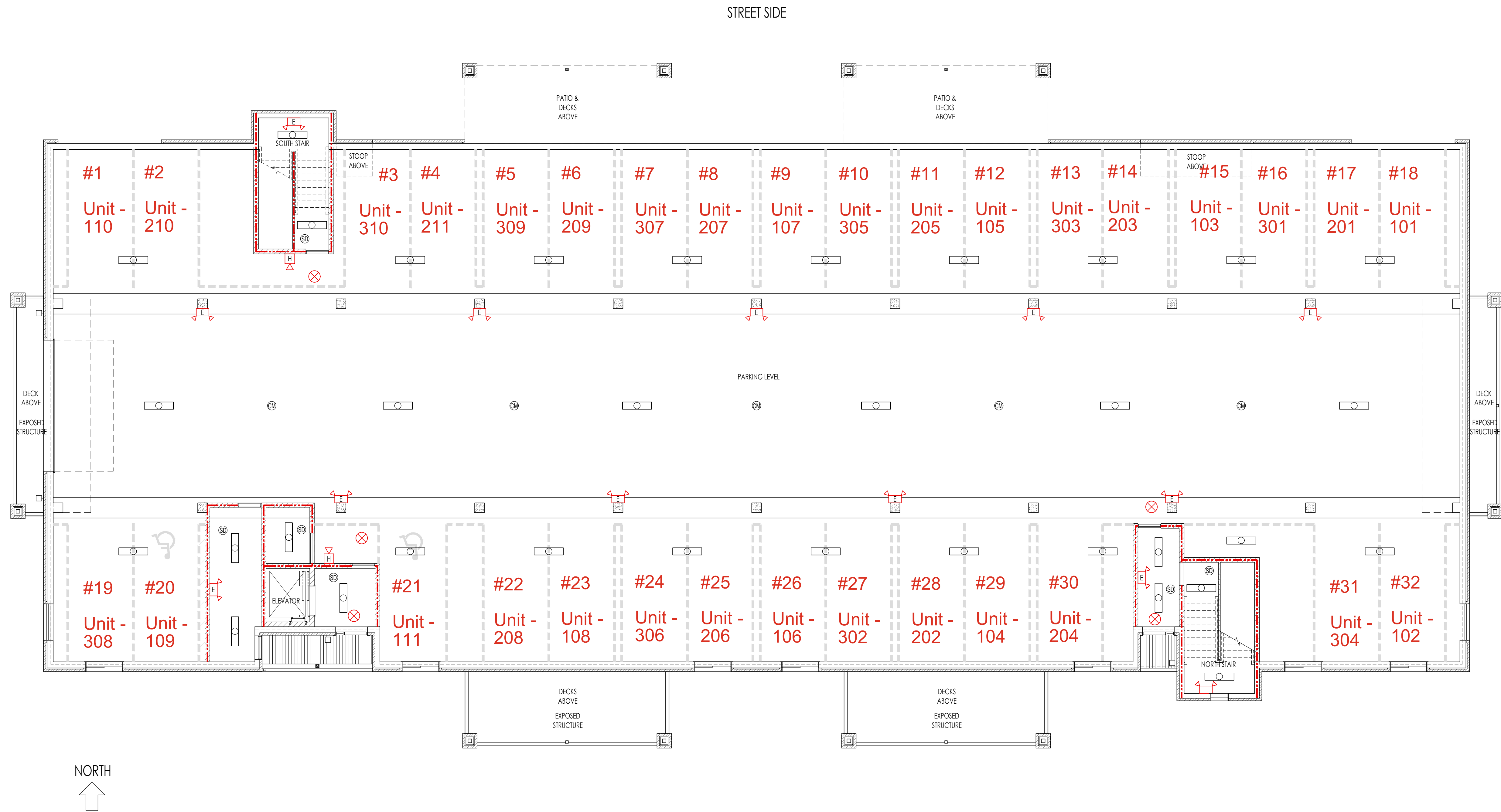
0 GROUND FLOOR REFLECTED CEILING PLAN 14,222 SQ. FT. Scale: 1/8" = 1'-0" --- = 1 HOUR FIRE RATED --- = 2 HOUR FIRE RATED
