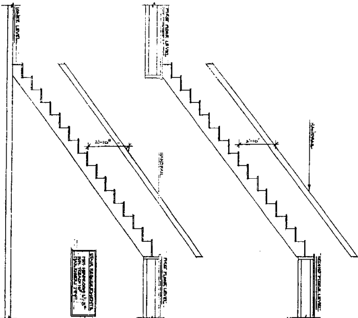
stair section
