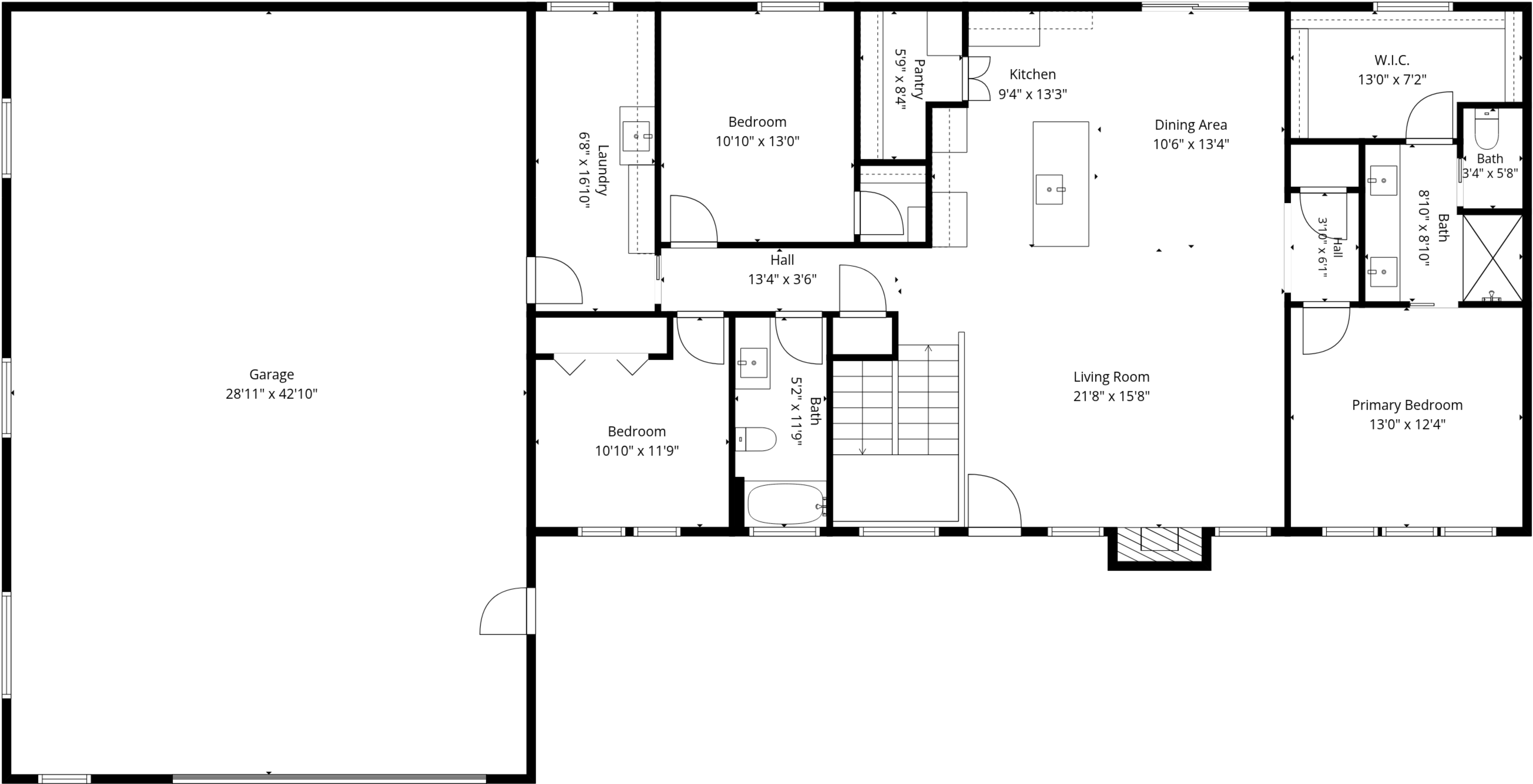
1st Floor
