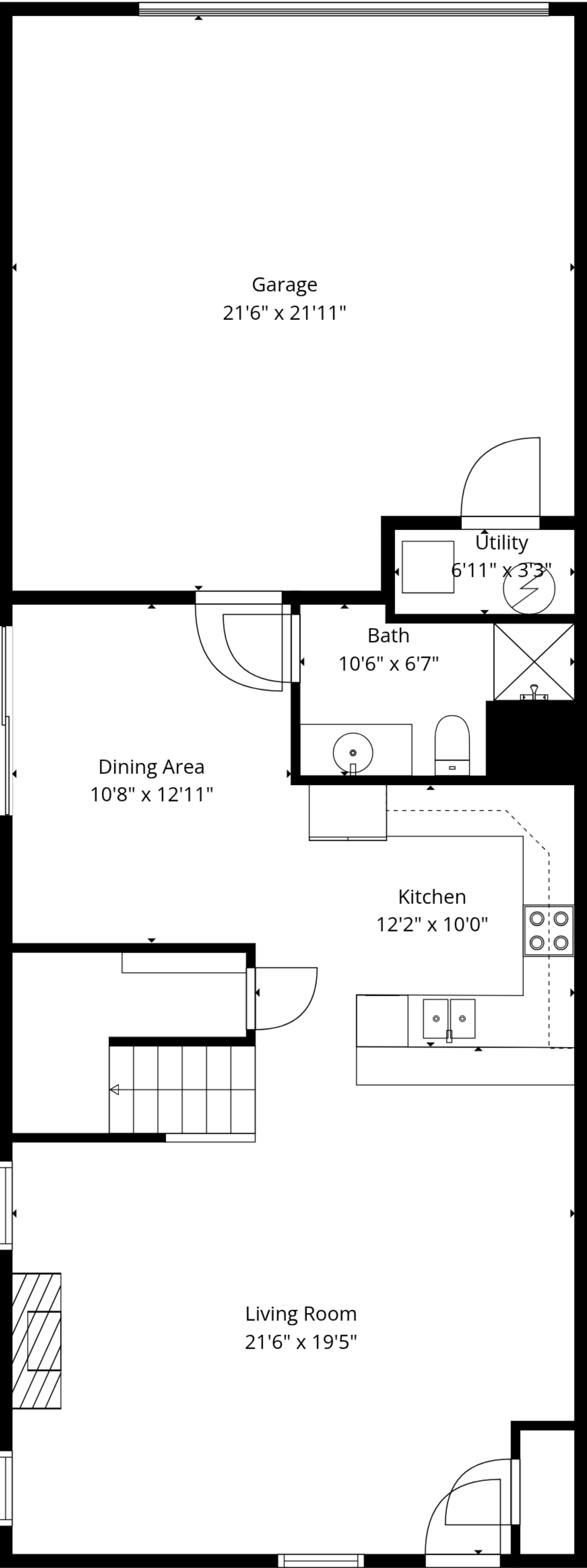
1st Floor
