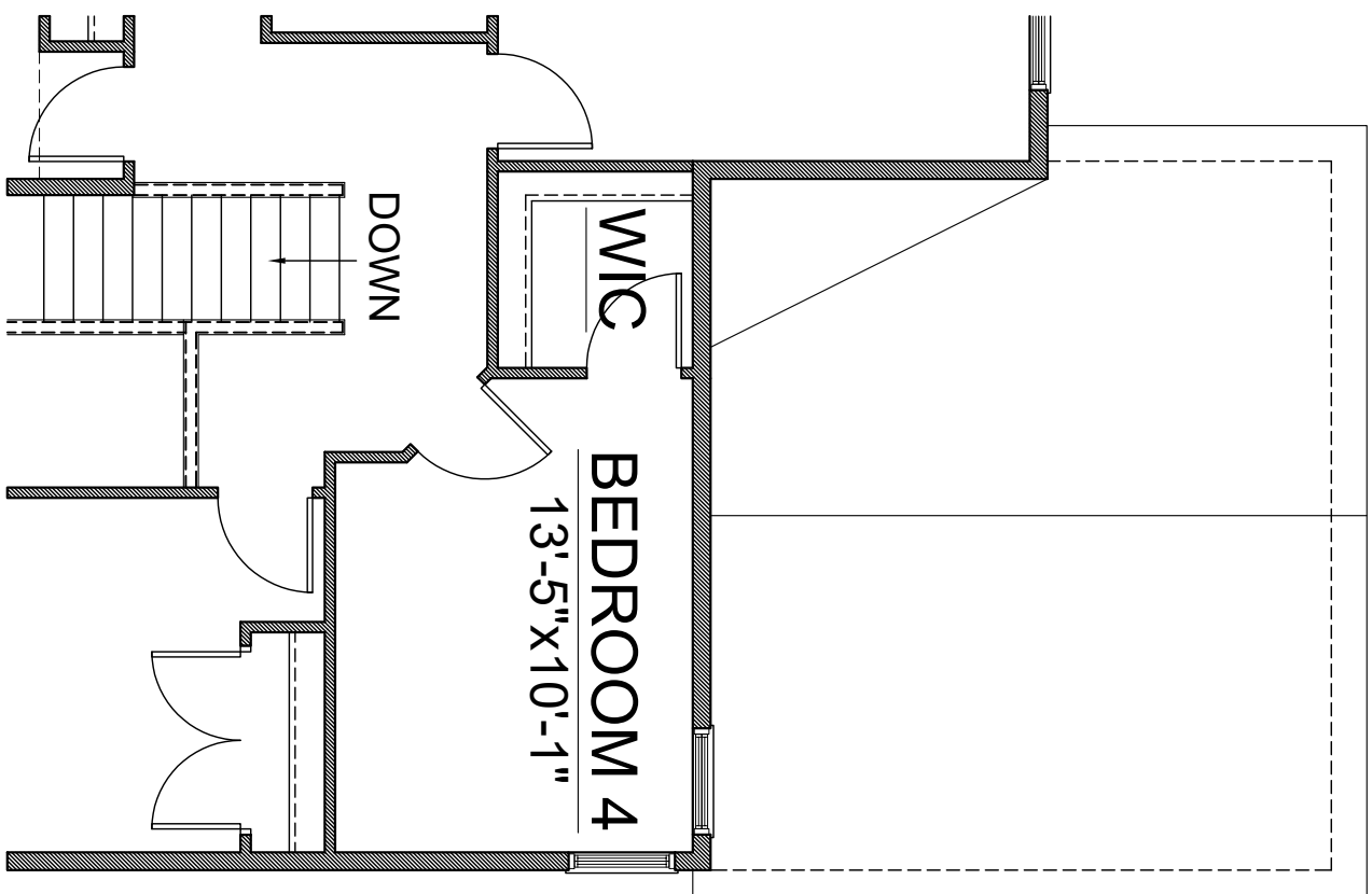
OPT. BEDROOM 4 PLAN
