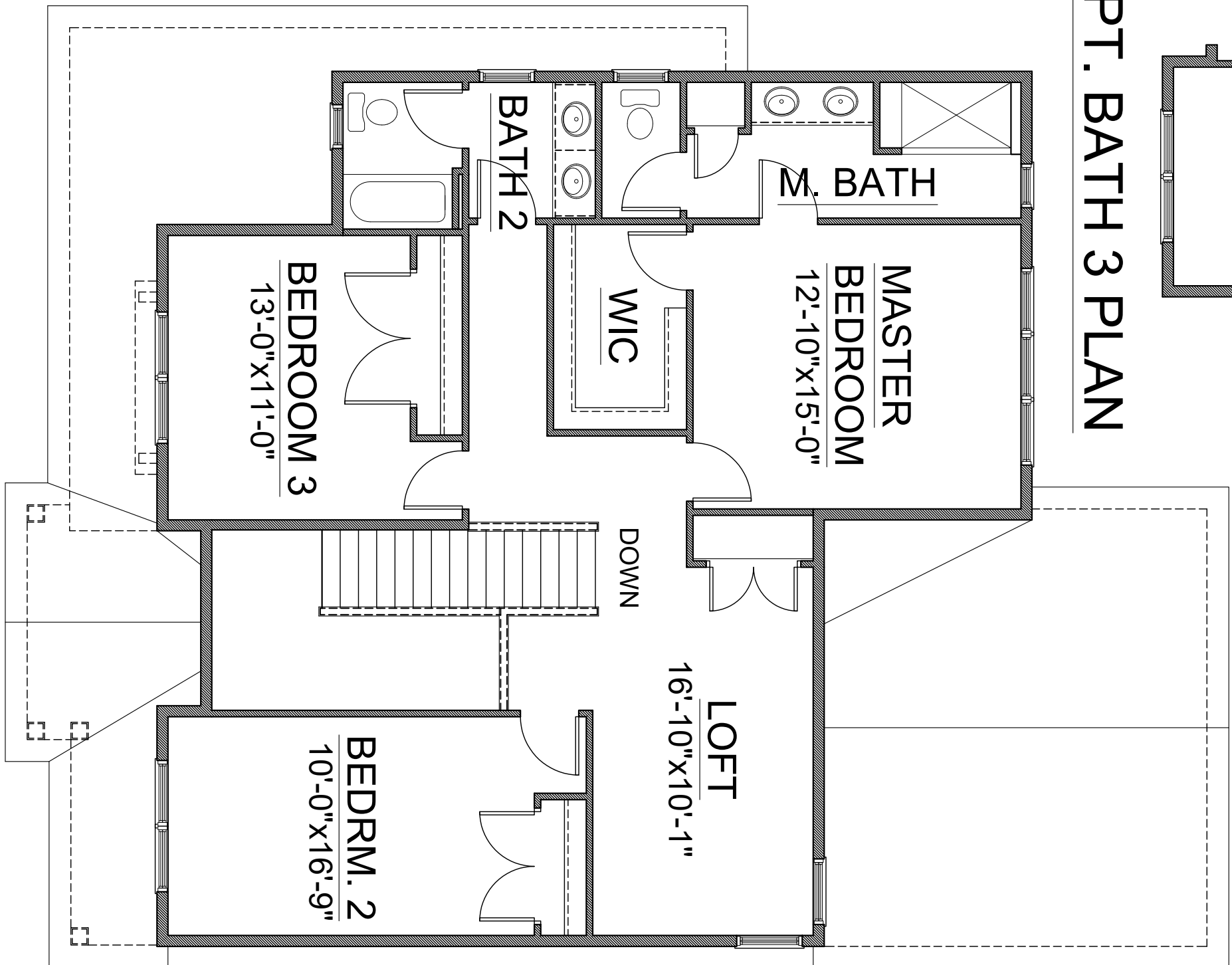
SECOND FLOOR PLAN - COTTAGE
