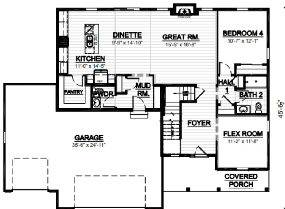
FIRST FLOOR LAYOUT
