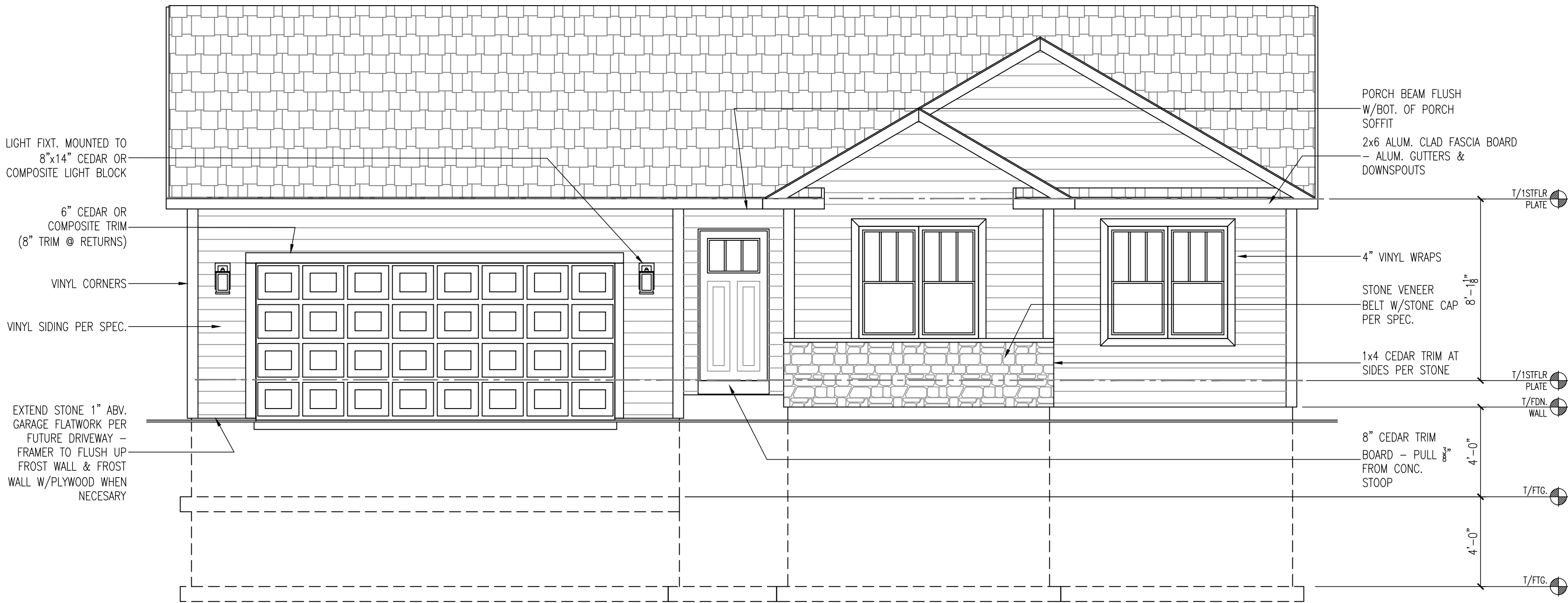
ELEVATION 1 FRONT ELEVATION SCALE: 1/4" = 1'-0"
