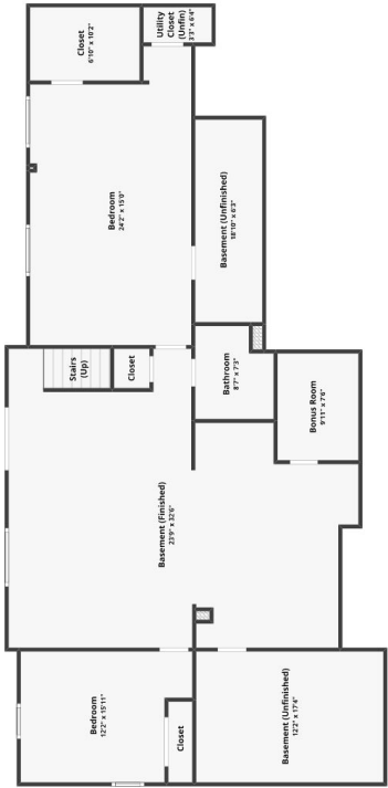
BASEMENT Finished area: ~1,476.89 sq. ft. Unfinished area: ~351.44 sq. ft.
