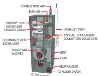
CONDENSATION IN A HIGH-EFFICIENCY FURNACE
