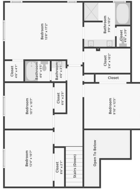
FLOOR 2
