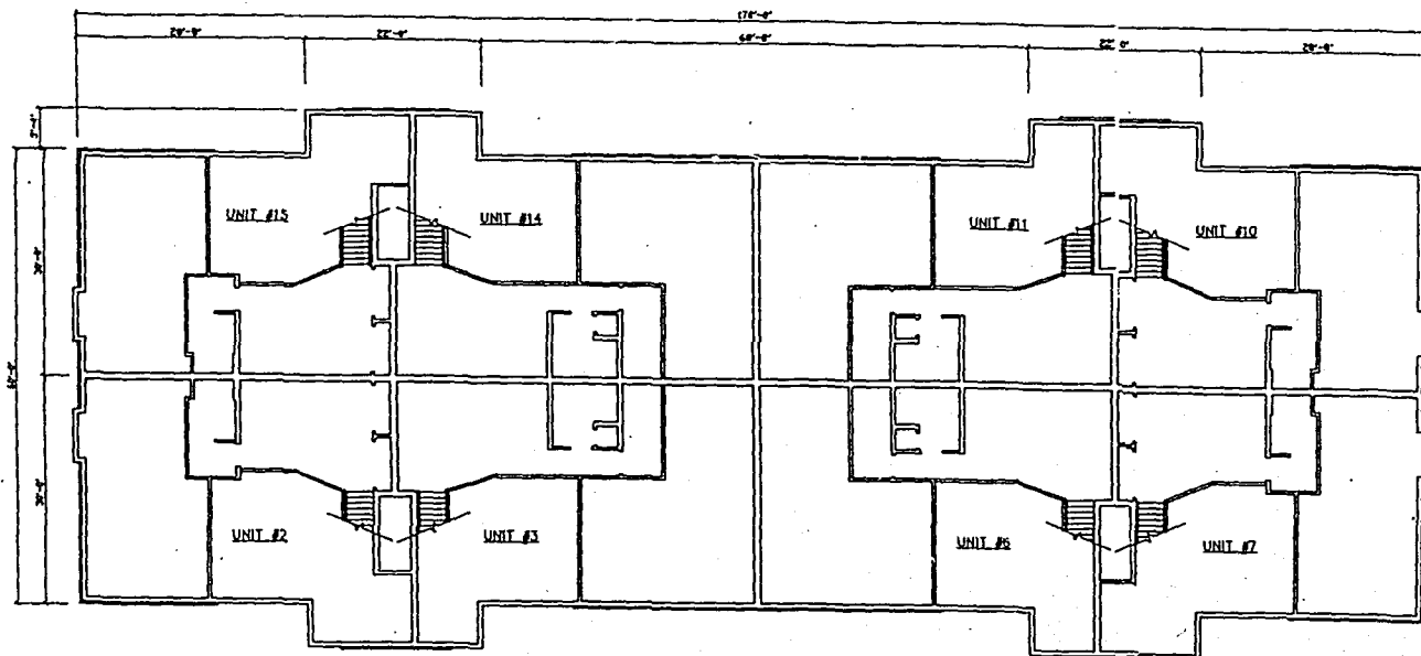
LOFT FLOOR PLAN 1/16" = 1'-0"
