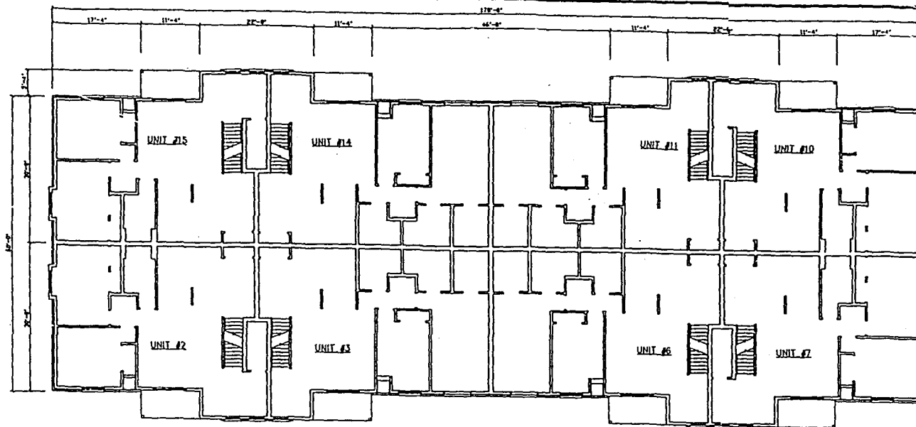
SECOND FLOOR PLAN 1/16" = 1'-0"
