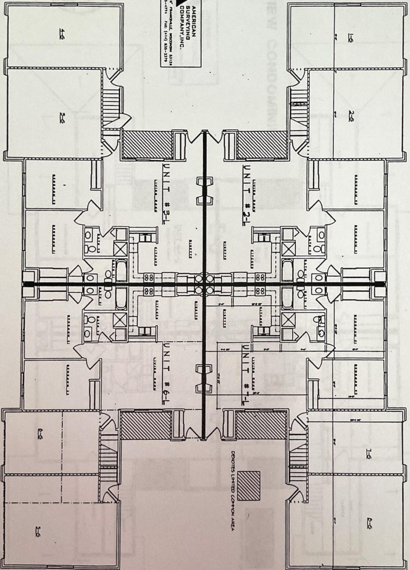
FIRST FLOOR PLAN FIRST FLOOR PLAN
