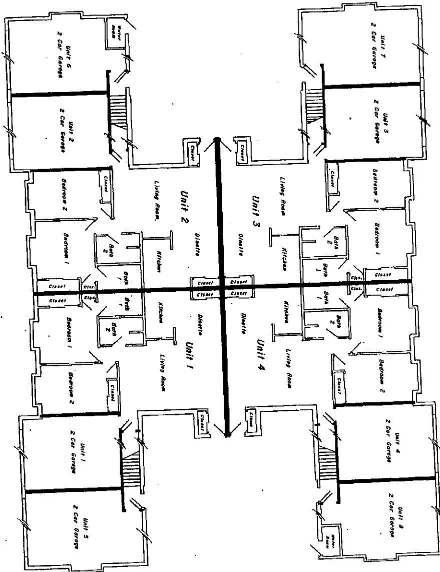
First Floor Plan (Bldgs. 1, 2, 3, 9 & 10) Scale: 1"=10'
