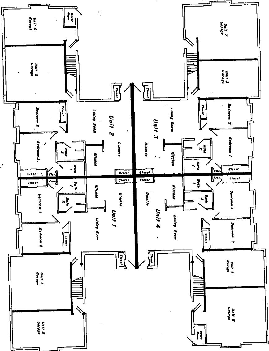
First Floor Plan (Blgs. 16, 17 & 18) Scale: 1" = 10'
