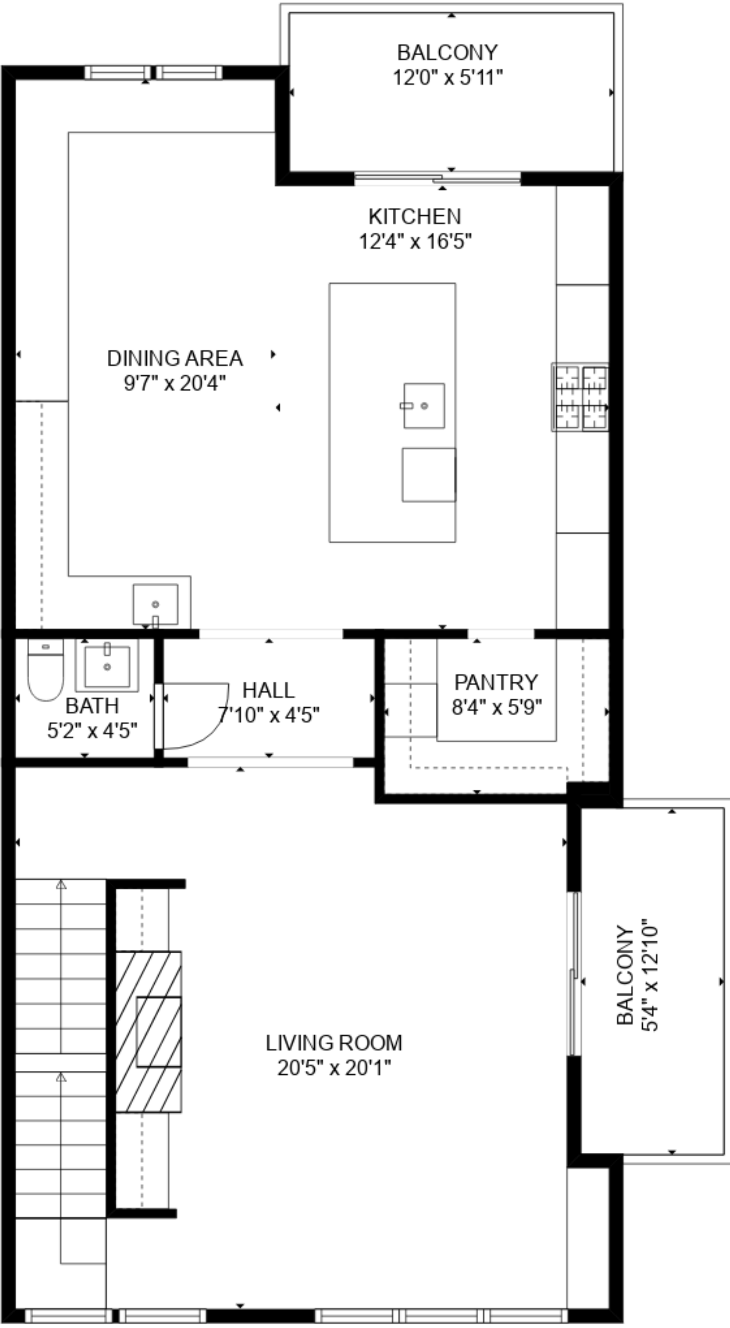
FLOOR 2
