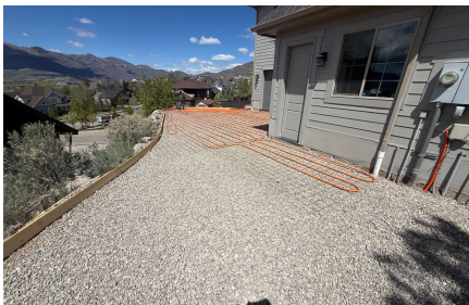
INSTALLATION PHOTOS - RADIANT TUBING PRIOR TO CONCRETE PLACEMENT
