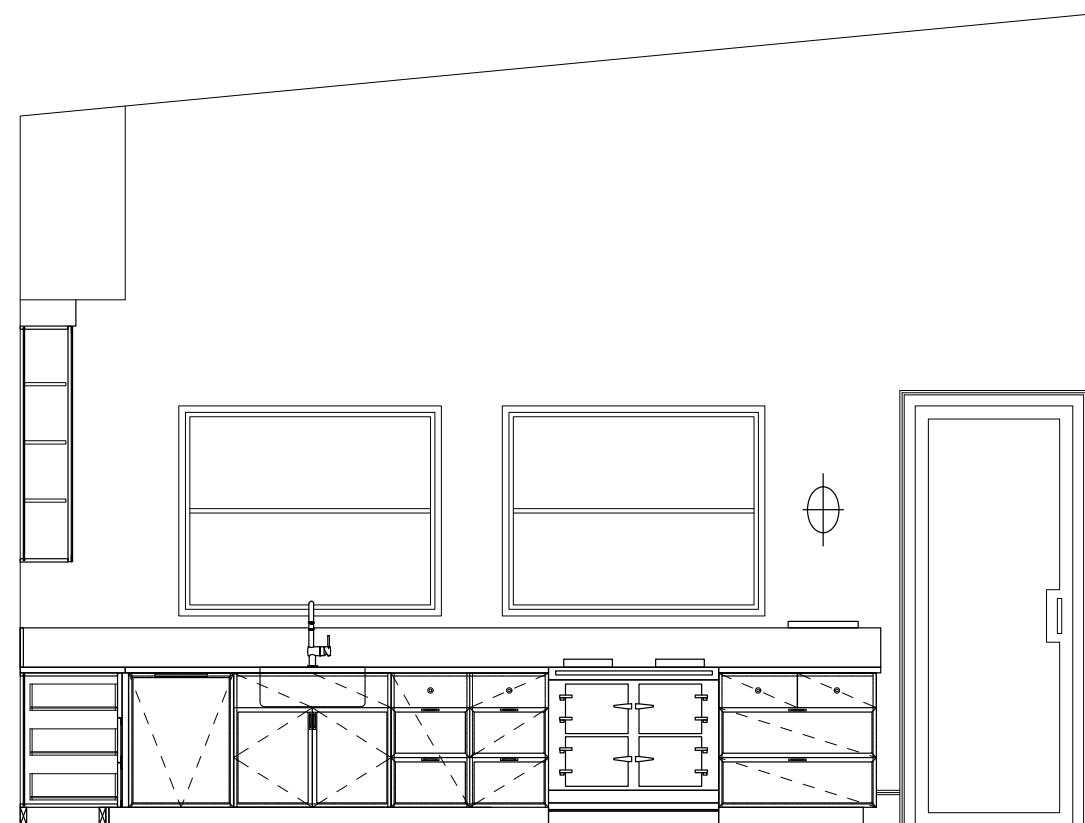
Sink Elevation
