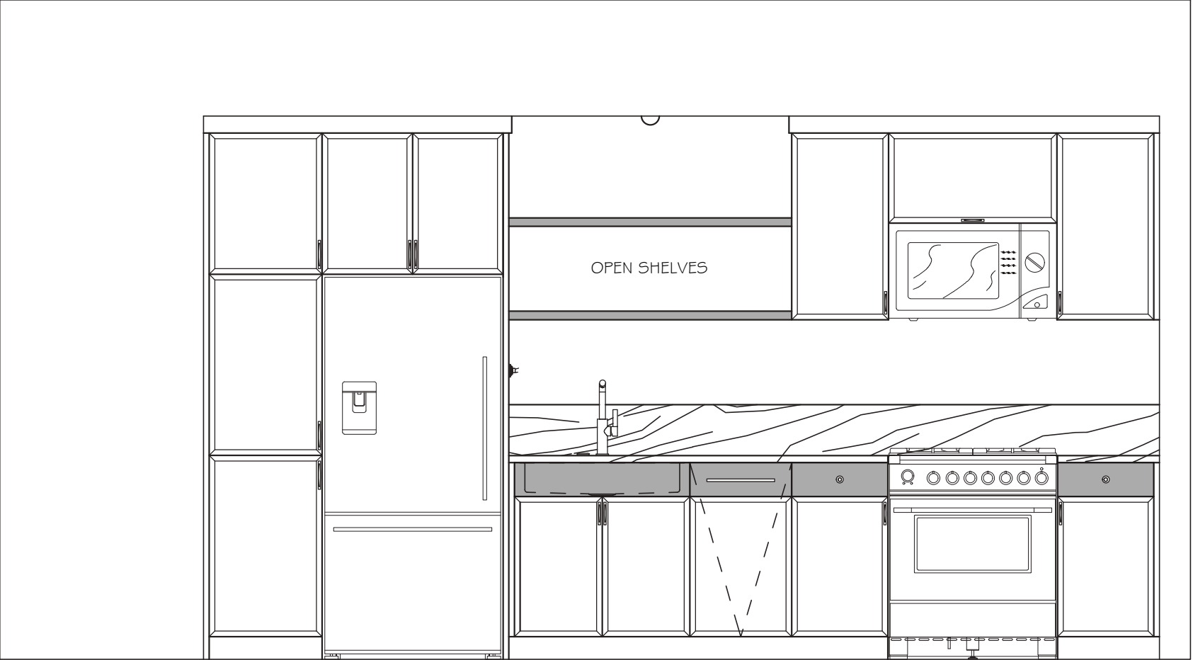
Kitchenette Elevation
