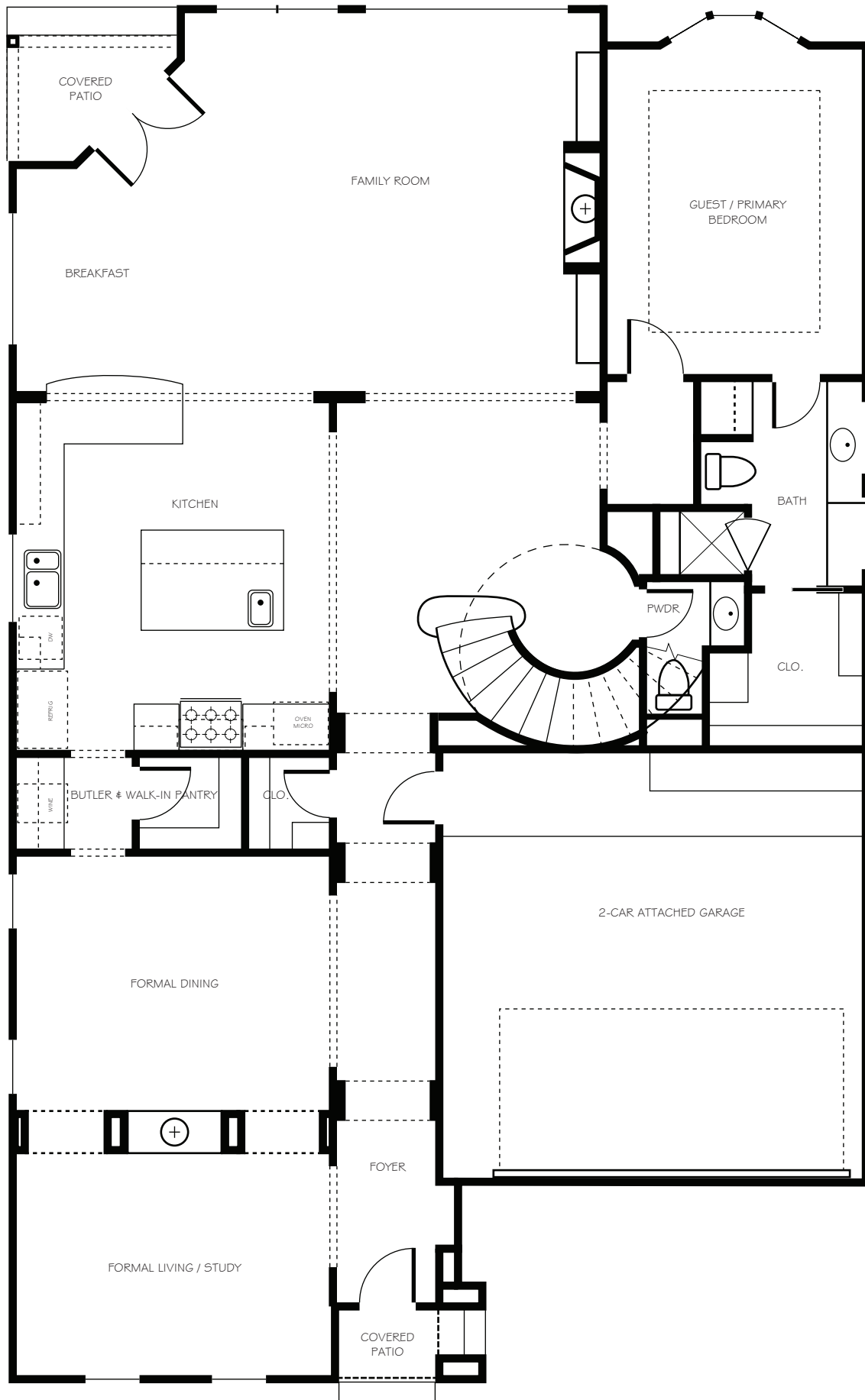
First Floor
