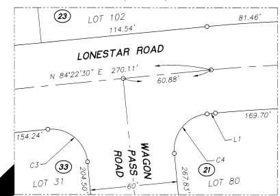
DETAIL VIEW "A" (NOT TO SCALE)
