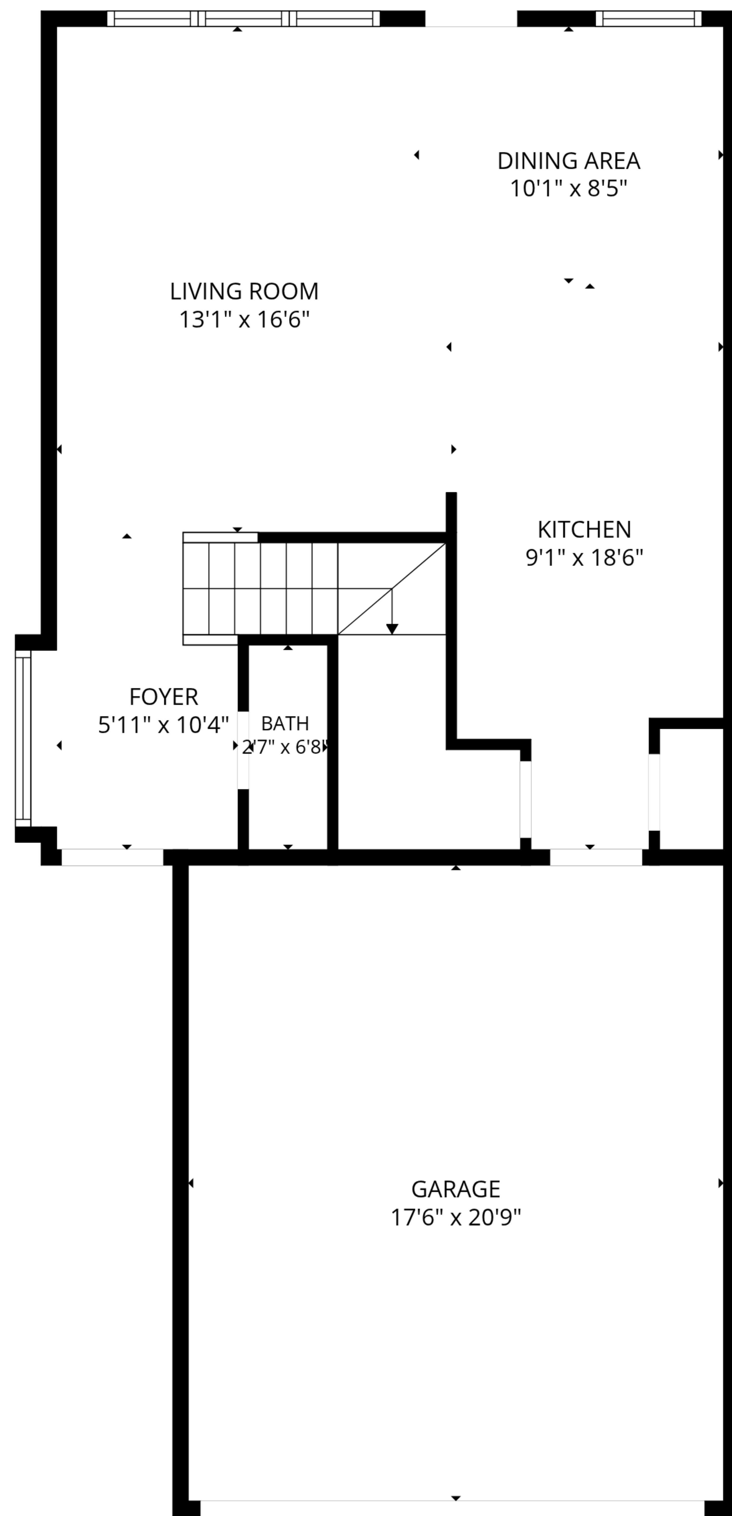
1st floor
