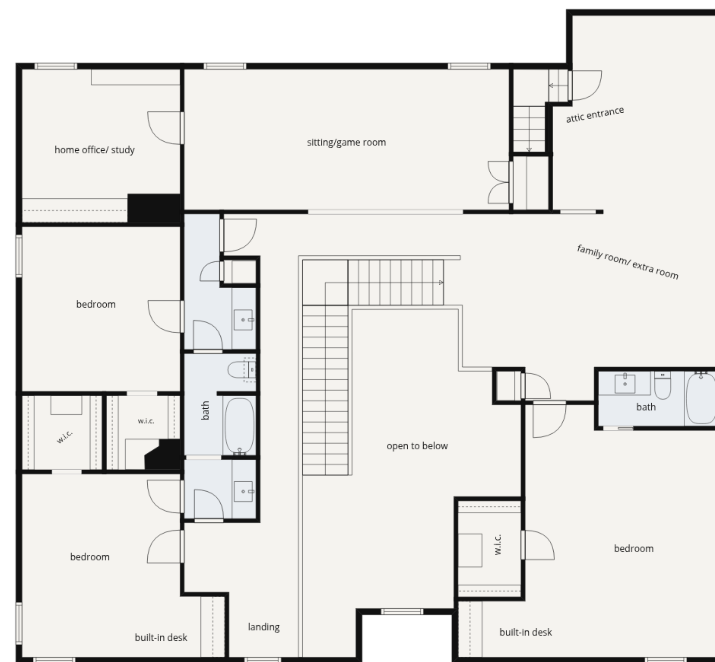
2nd floor
