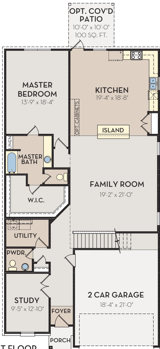
FIRST FLOOR
