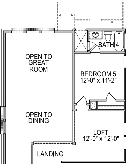
SECOND FLOOR PLAN OPT. #0094 BED 5/ BATH 4 FROM STORAGE
