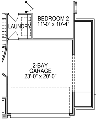
FIRST FLOOR PLAN OPT. #0613 5' GARAGE EXT.
