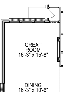
FIRST FLOOR PLAN OPT. #FRESC501 ELECTRIC FIREPLACE
