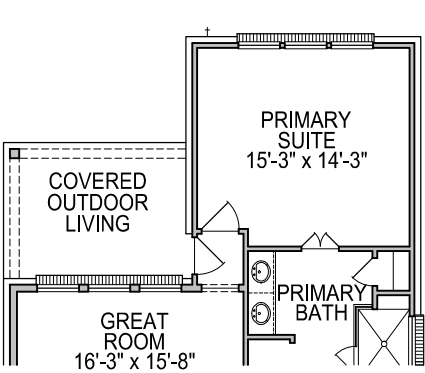
FIRST FLOOR PLAN OPT. #0105 COVERED OUTDOOR LIVING
