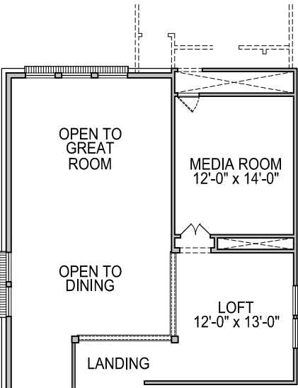
SECOND FLOOR PLAN OPT. #0526 MEDIA ROOM FROM STORAGE
