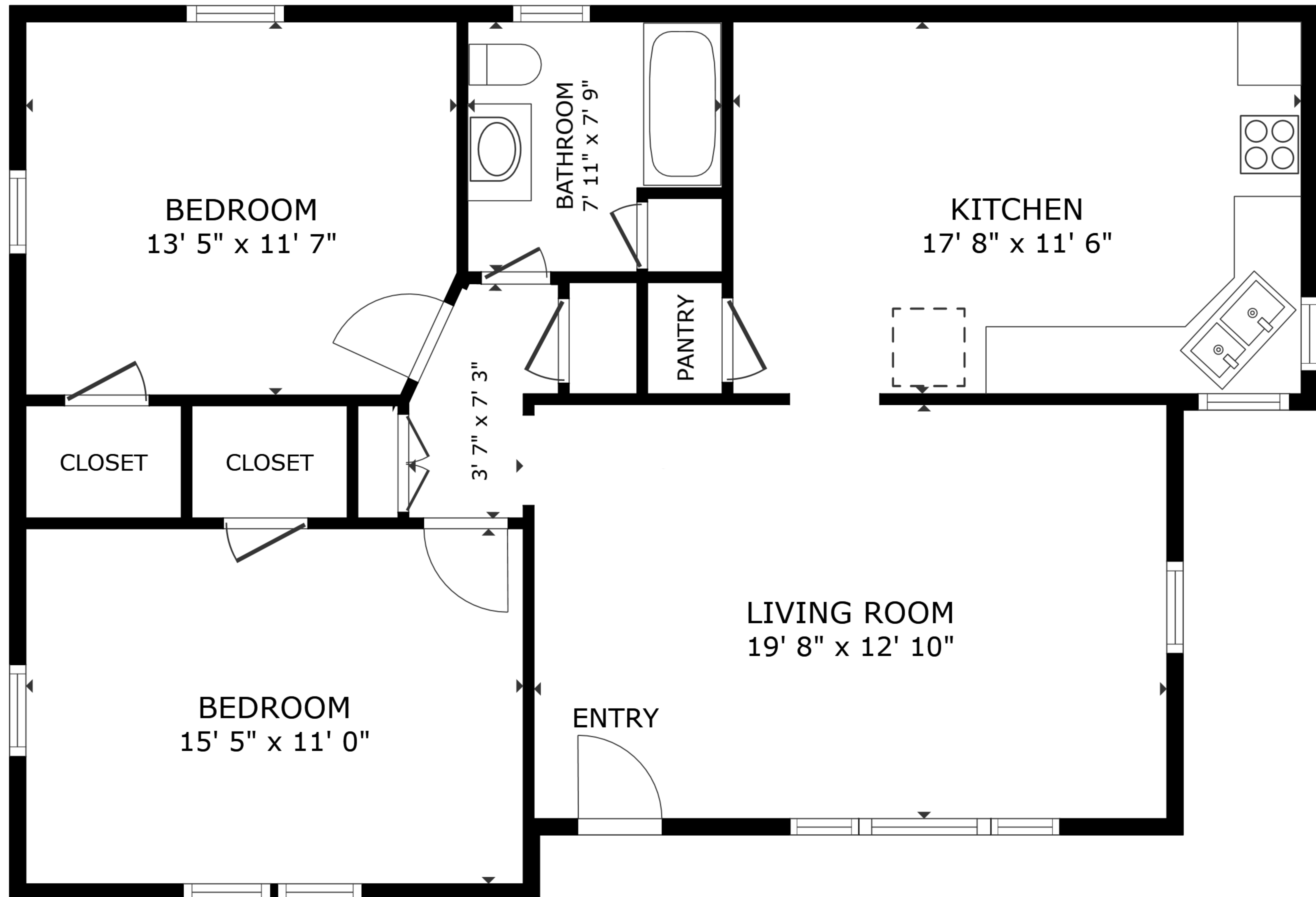
FLOOR PLAN
