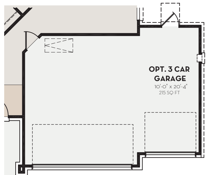
OPT. 3 CAR GARAGE
