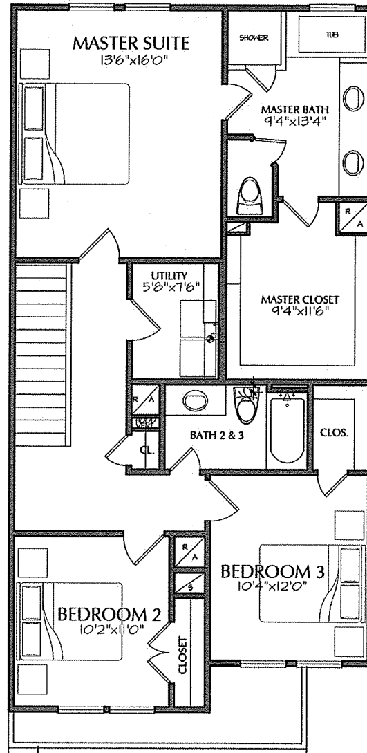
SECOND FLOOR
