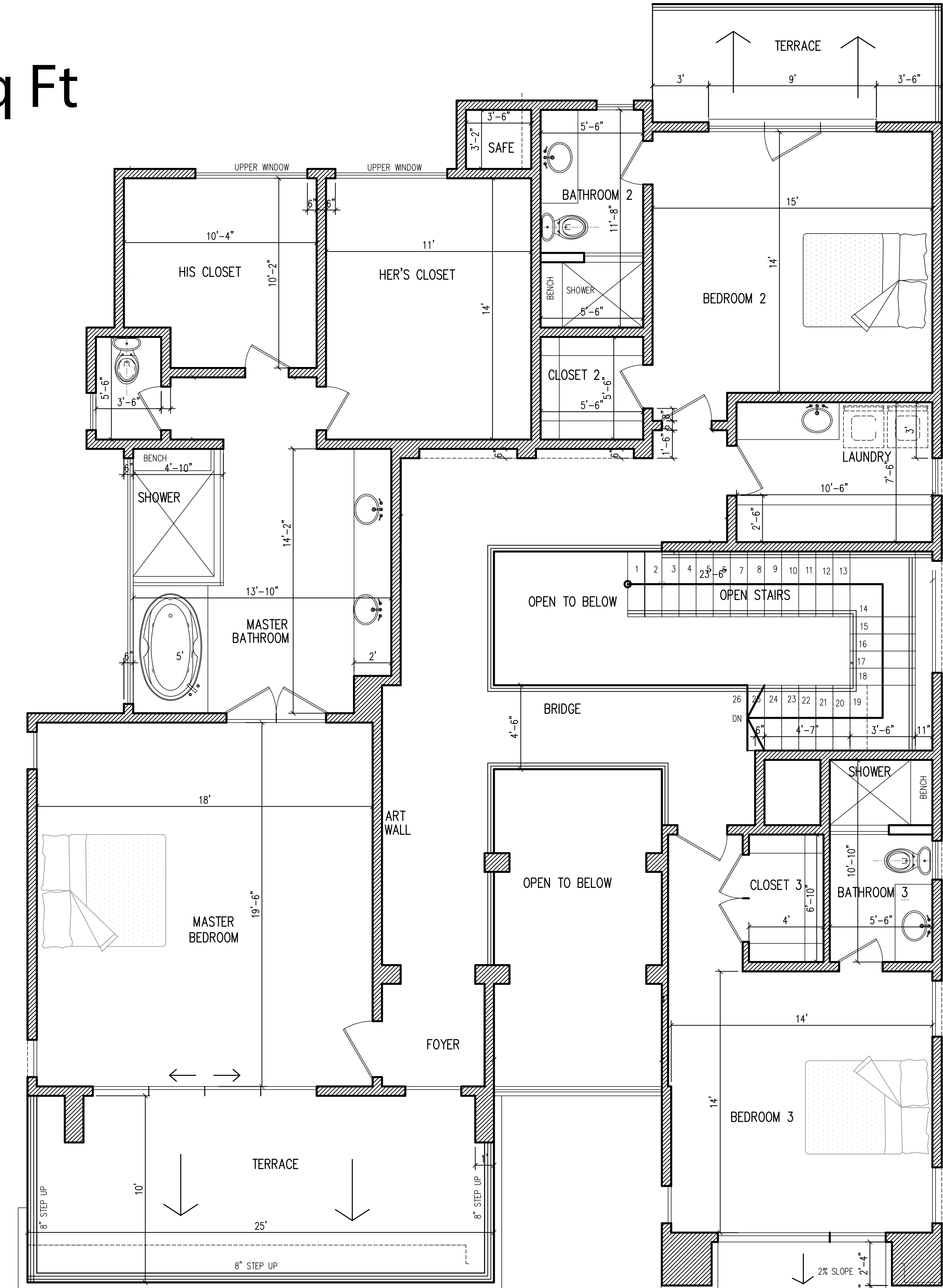
Second Floor
