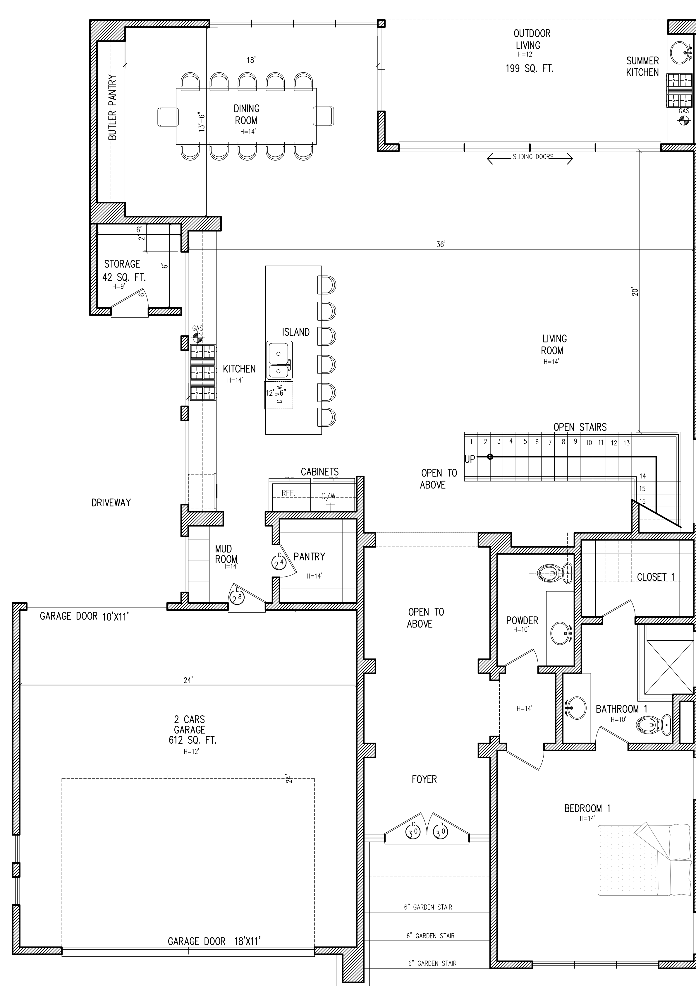
First Floor
