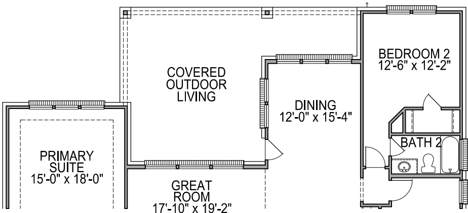
FIRST FLOOR PLAN OPT. #367 EXTENDED COVERED OUTDOOR LIVING
