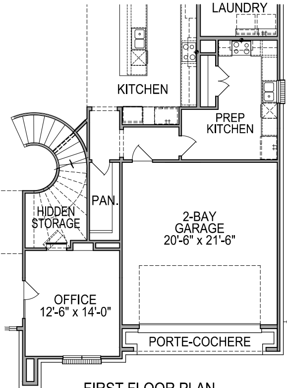
FIRST FLOOR PLAN OPT. #0485 PREP. KITCHEN FROM GARAGE
