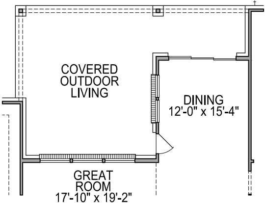
FIRST FLOOR PLAN OPT. #0798 EXT. COVERED OUTDOOR LIVING w/ SLIDERS @ DINING
