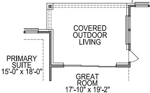
FIRST FLOOR PLAN OPT. #0790 SLIDERS @ GREAT ROOM
