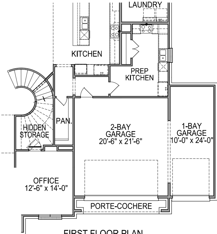
FIRST FLOOR PLAN OPT. #0485 PREP. KITCHEN w/ #0593 1 BAY GARAGE FROM GARAGE
