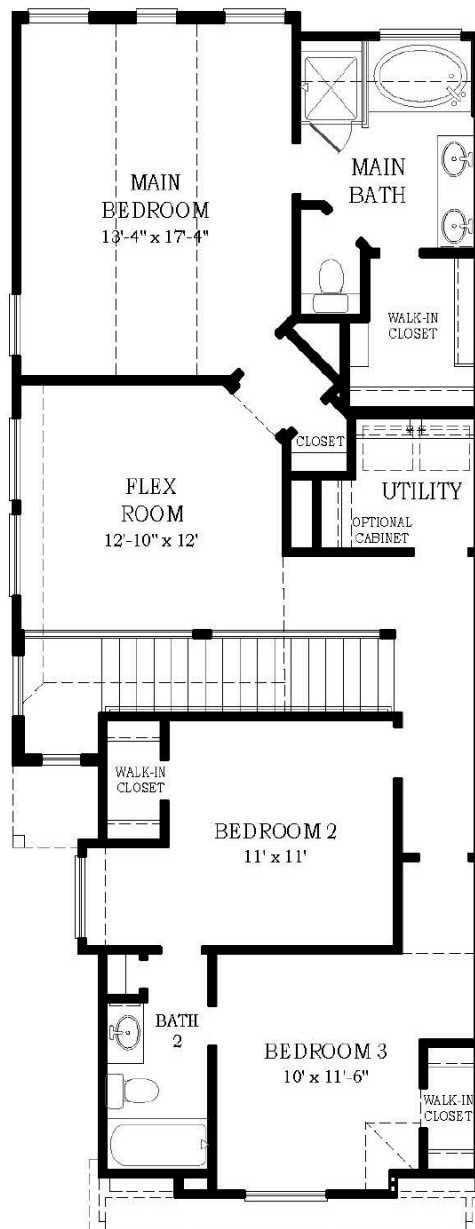
SECOND FLOOR
