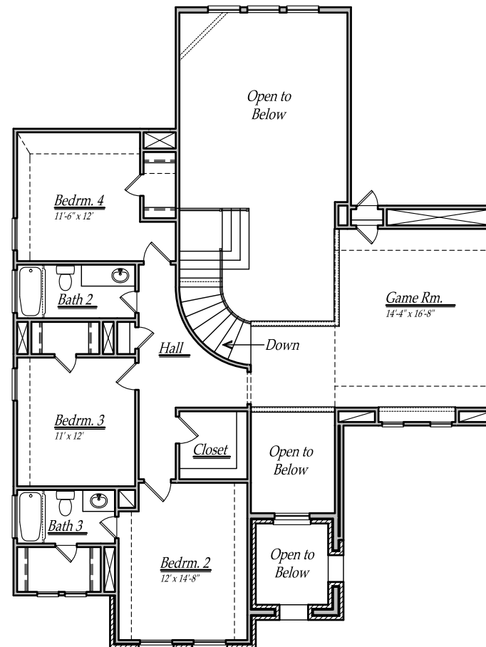
Second Floor
