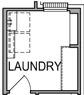
FIRST FLOOR PLAN OPT. #0152 LAUNDRY CABINETS
