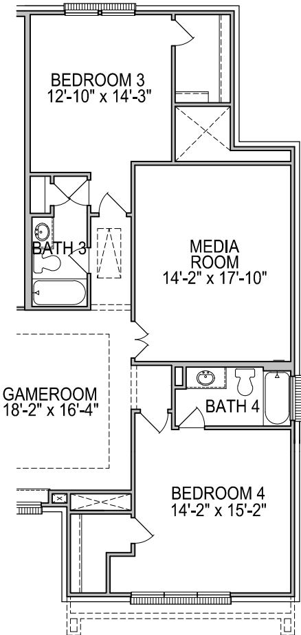
SECOND FLOOR PLAN OPT. #0612 MEDIA ROOM FROM BEDROOM 5
