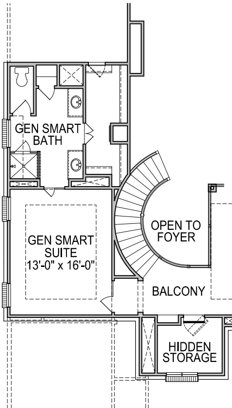
SECOND FLOOR PLAN OPT. #0476 GEN SMART SUITE FROM ATTIC SPACE
