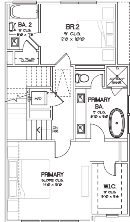
THIRD FLOOR
