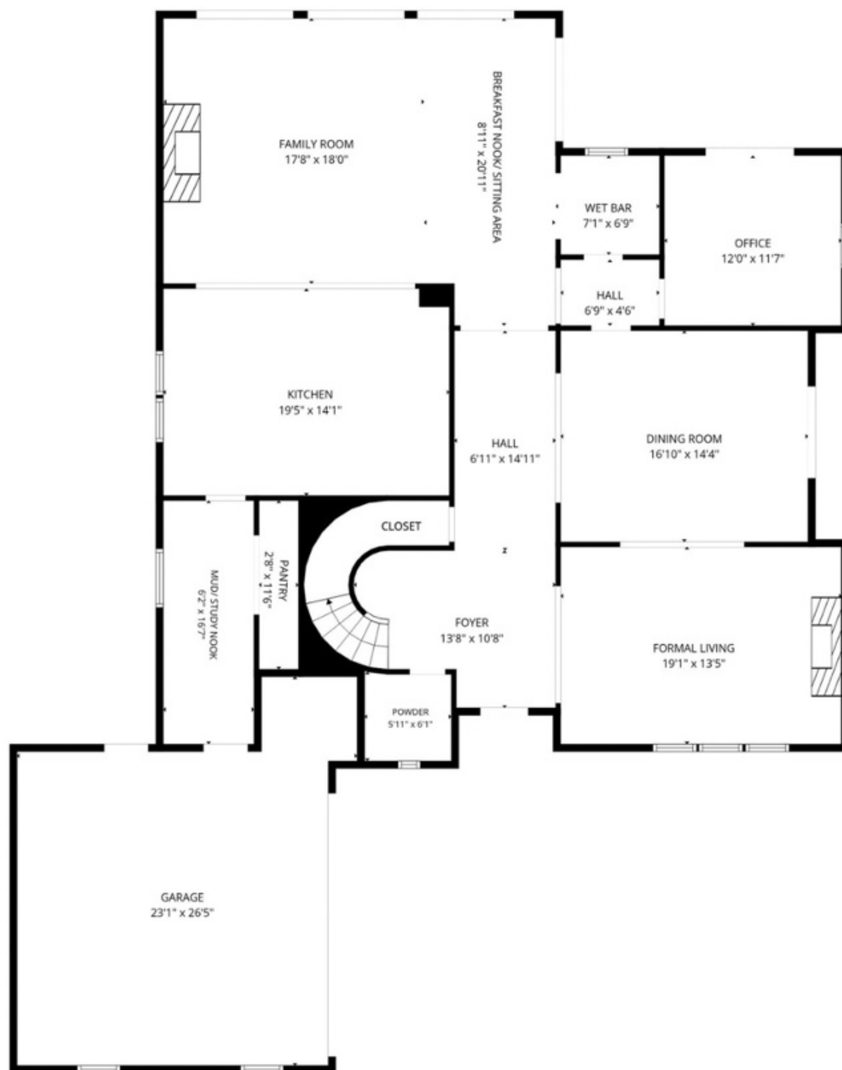
1st floor
