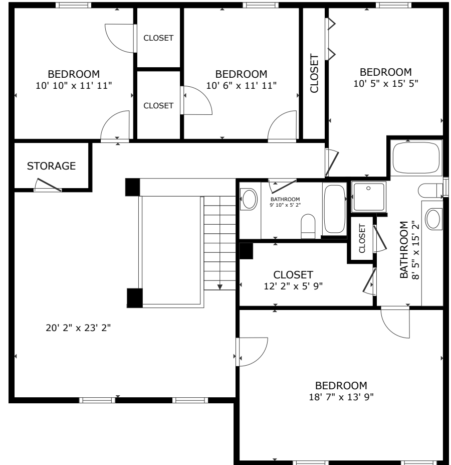
FLOOR 2
