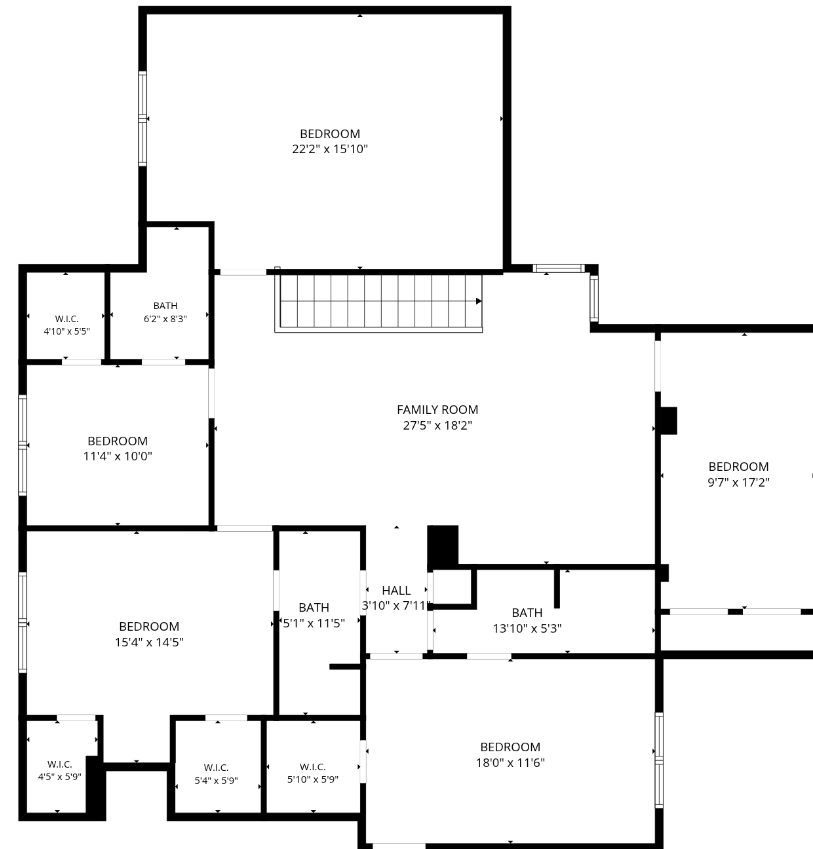
2nd floor
