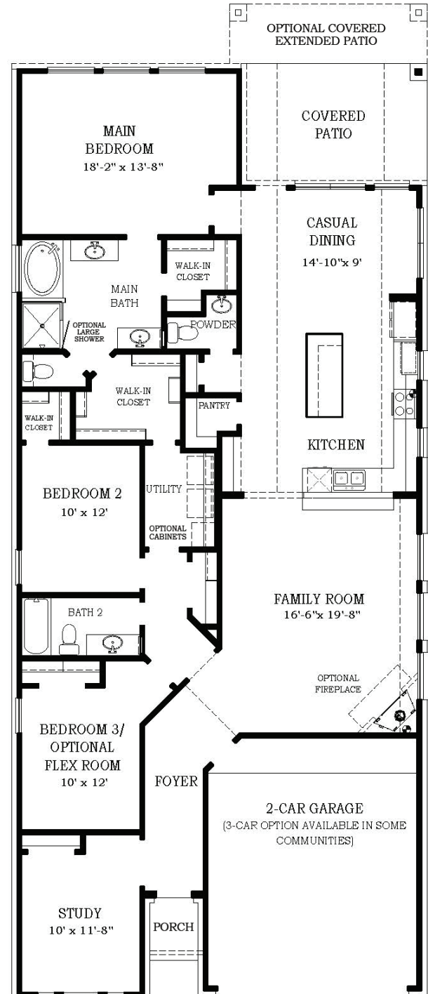
FLOOR PLAN
