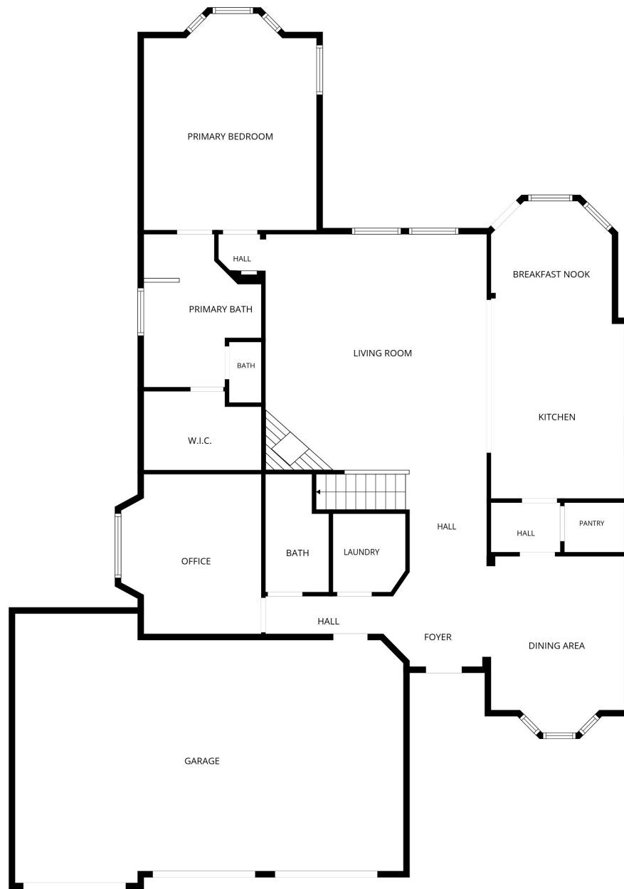
1st floor
