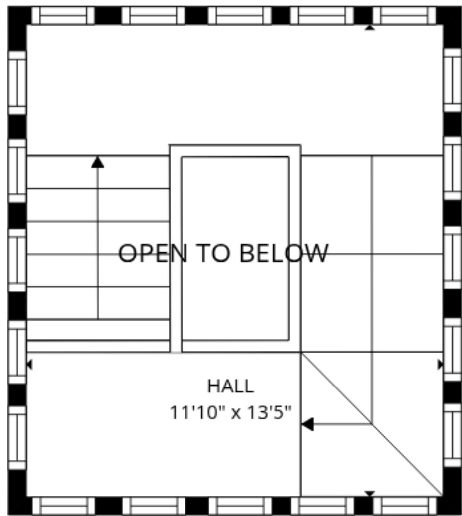
3rd floor
