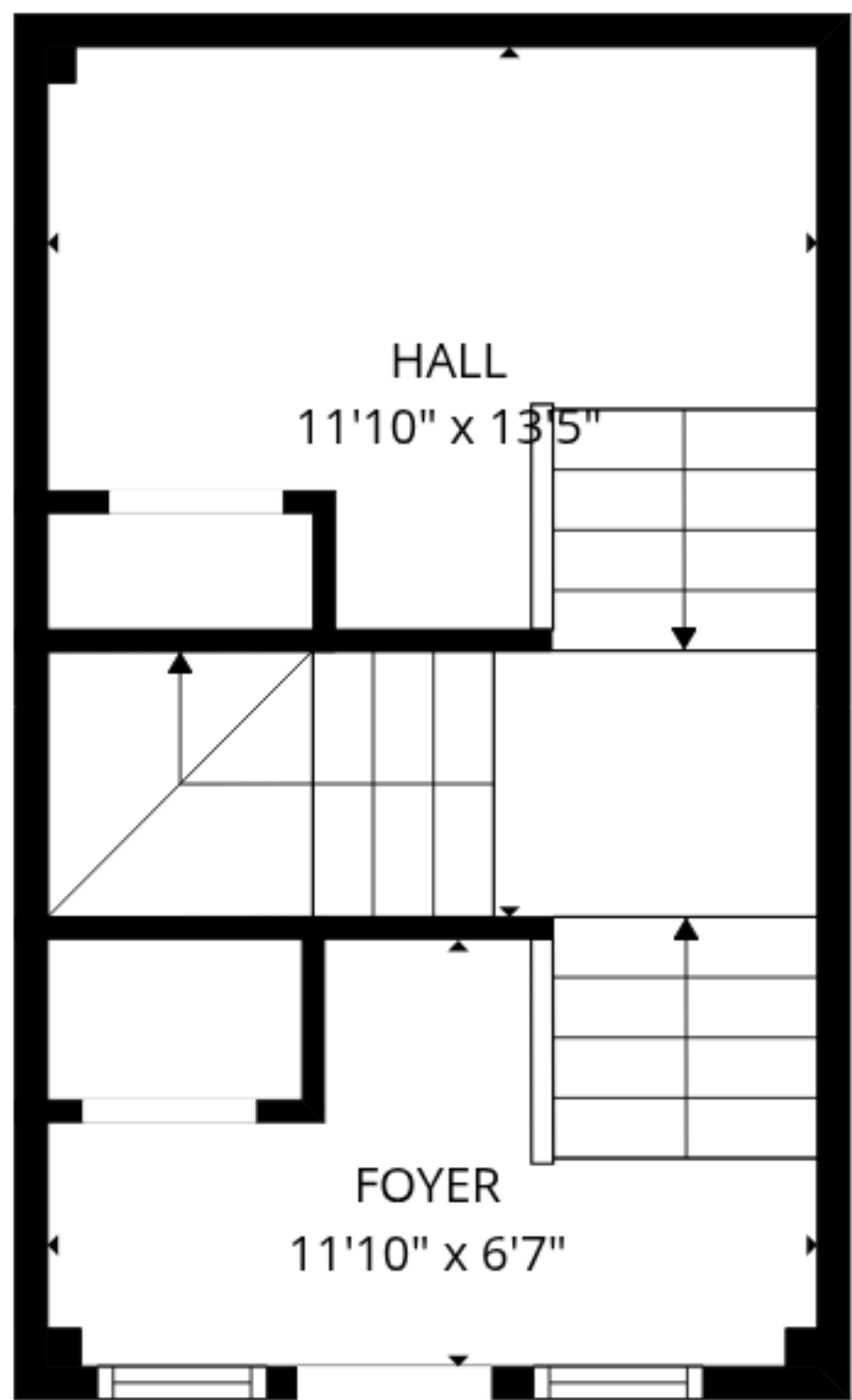
Basement
