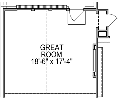
FIRST FLOOR PLAN OPT. #FRESC501 ELECTRIC FIREPLACE
