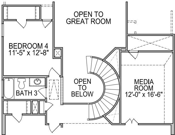
2nd FLOOR PLAN OPT. #0113 CURVED STAIRS w/ #0526 MEDIA ROOM
