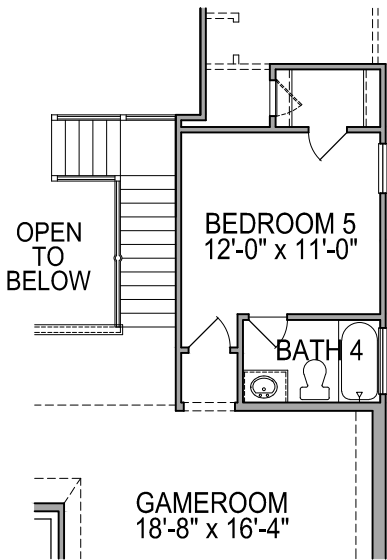
SECOND FLOOR PLAN OPT. #0094 BED 5/BATH 4 FROM ATTIC
