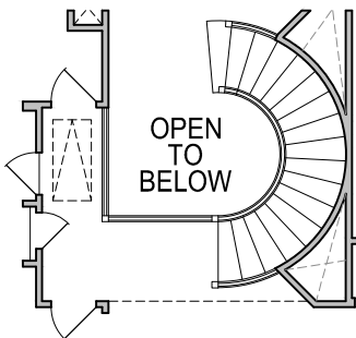
2nd FLOOR PLAN OPT. #0050 RAILING w/ #0113 CURVED STAIRS
