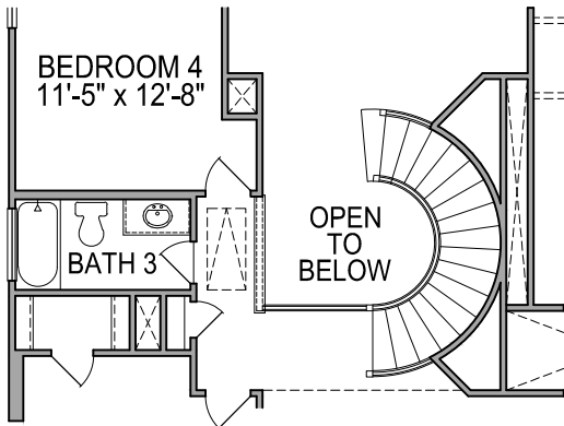
SECOND FLOOR PLAN OPT. #0113 CURVED STAIRS
