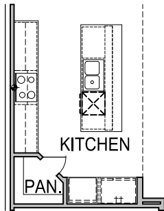
FIRST FLOOR PLAN OPT. #KITUPGSI 36" COOKTOP w/ OVEN/MICRO TOWER CONFIGURATION
