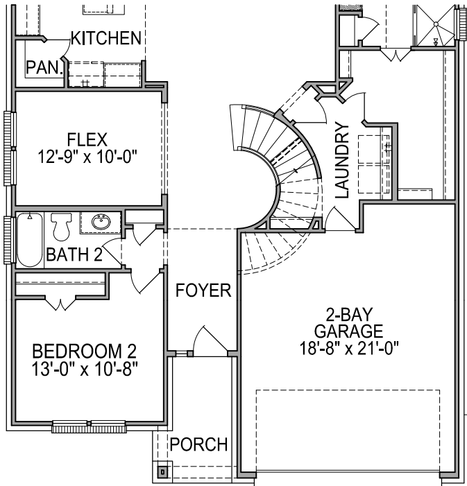
FIRST FLOOR PLAN OPT. #0113 CURVED STAIRS
