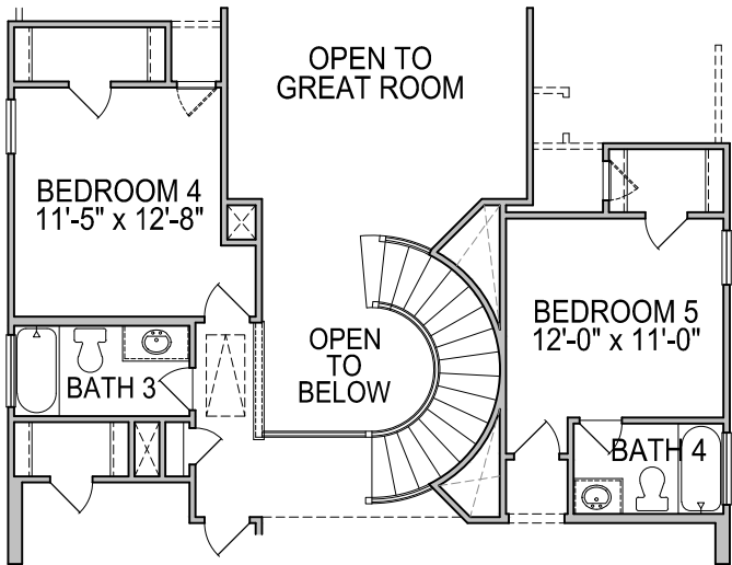
2nd FLOOR PLAN OPT. #0113 CURVED STAIRS w/ #0094 BED 5/BATH 4
