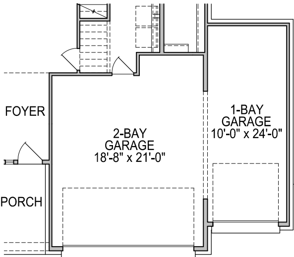
FIRST FLOOR PLAN OPT. #0593 1 BAY GARAGE
