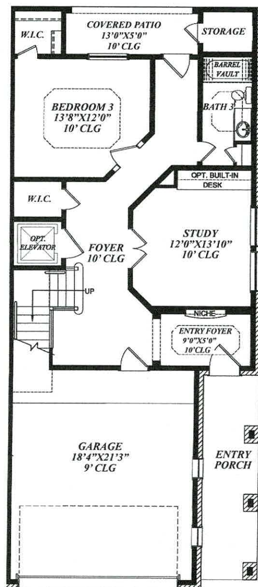
FIRST FLOOR
