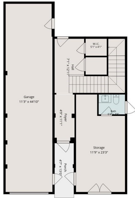
Basement
