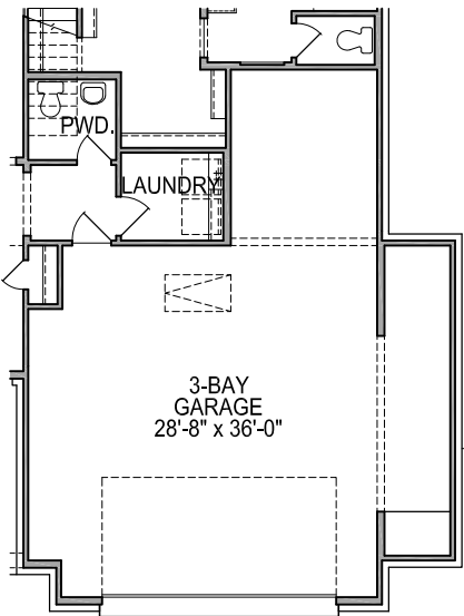
FIRST FLOOR PLAN OPT. #0613 5' GARAGE EXT.
