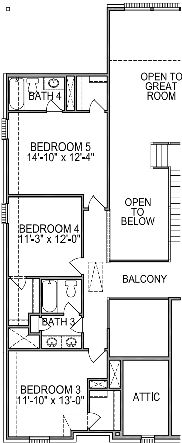
SECOND FLOOR PLAN OPT. #0094 BEDROOM 5/BATH 4 FROM ATTIC
