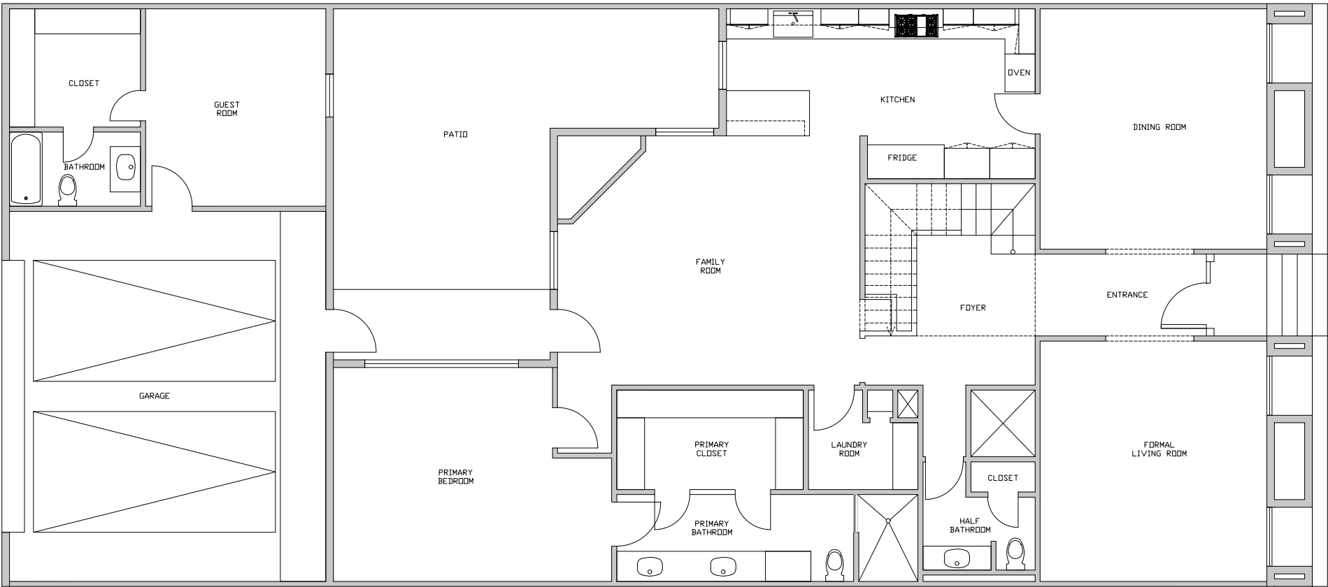
FIRST FLOOR LAYOUT PLAN
