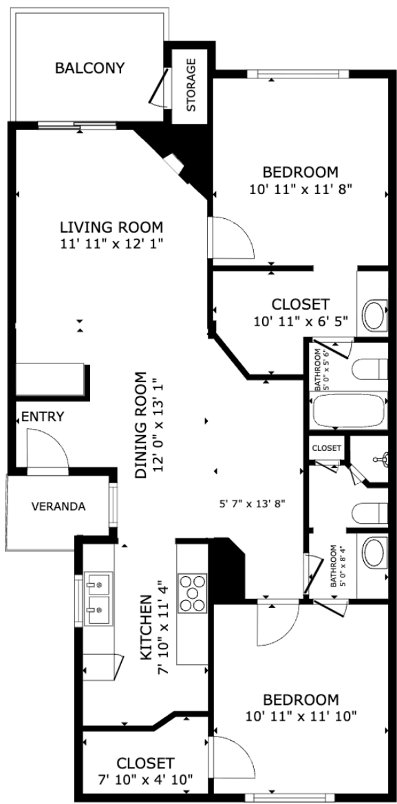
FLOOR PLAN
