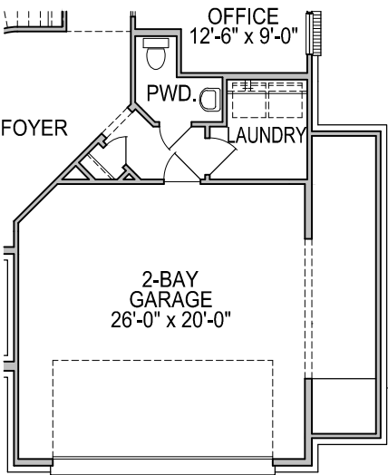
FIRST FLOOR PLAN OPT. #0613 5' GARAGE EXT.
