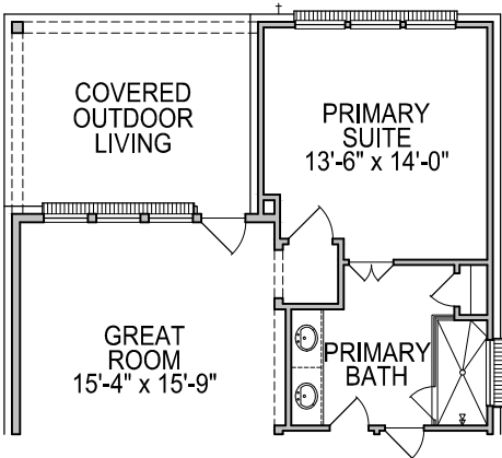
FIRST FLOOR PLAN OPT. #0105 COVERED OUTDOOR LIVING
