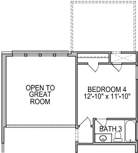
SECOND FLOOR PLAN OPT. #0178 BATH 3
