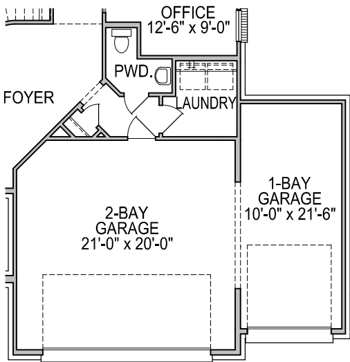
FIRST FLOOR PLAN OPT. #0593 1 BAY GARAGE
