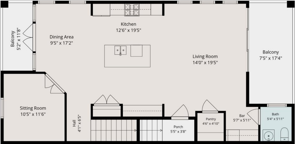
1st Floor
