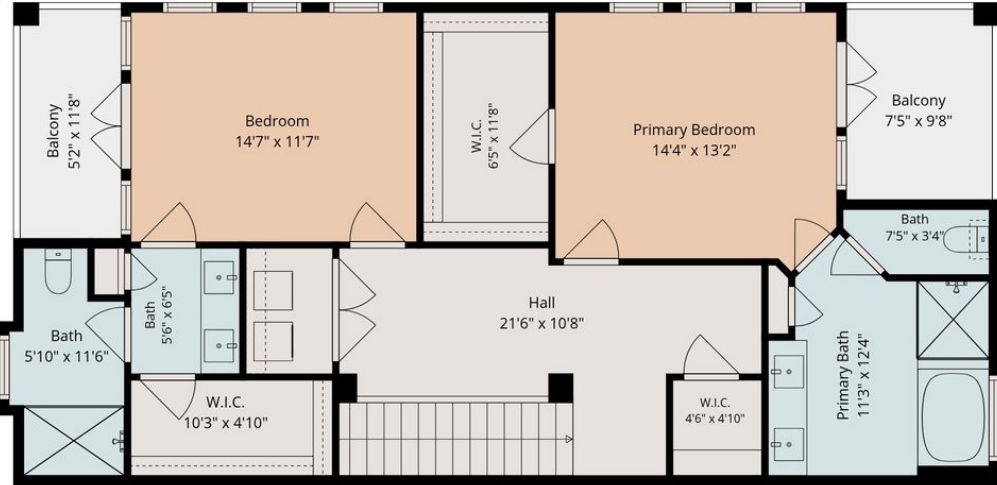
2nd Floor
