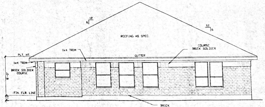
rear elevation
