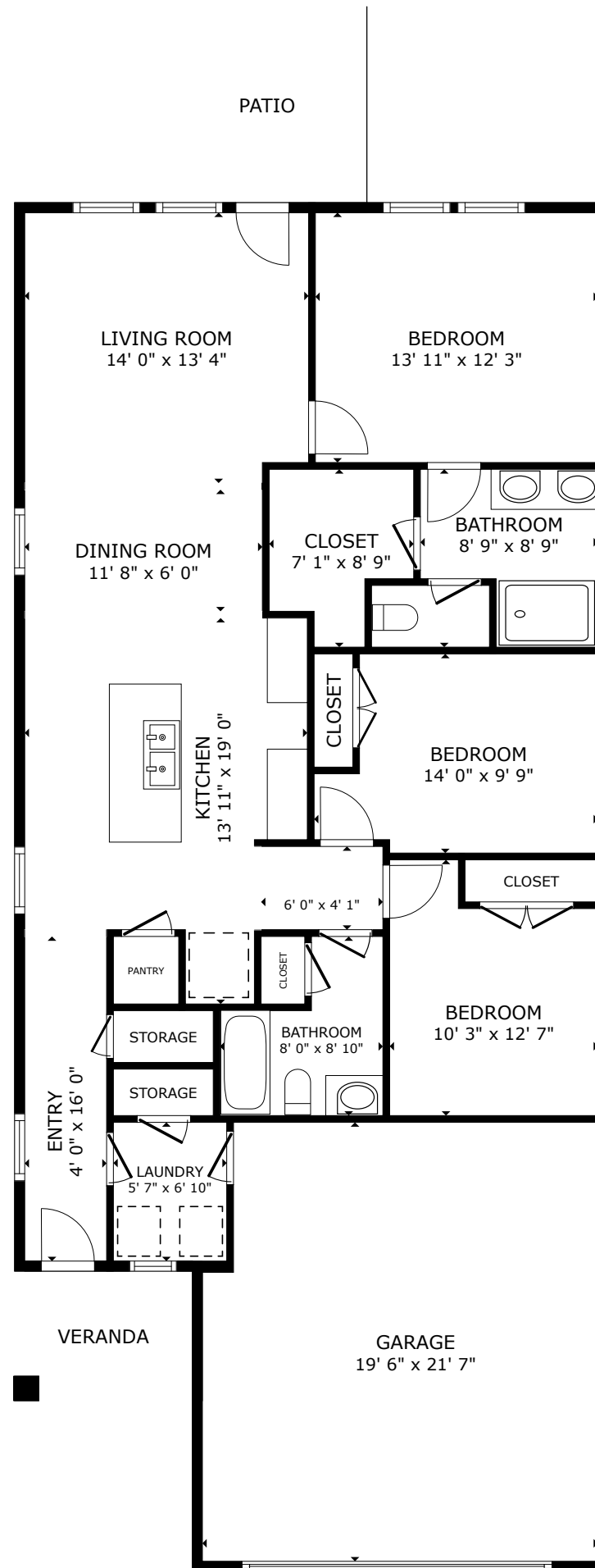
FLOOR PLAN
