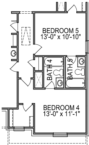
SECOND FLOOR PLAN OPT. #0567 BATH 5 FROM BATH 4
