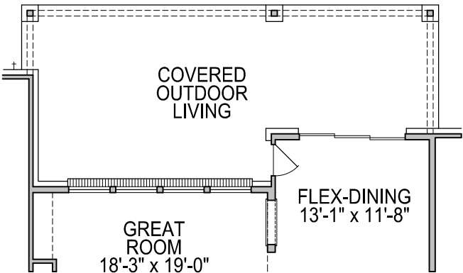
FIRST FLOOR PLAN OPT. #0789 EXT. COVERED OUTDOOR LIVING W/ SLIDERS @ FLEX-DINING
