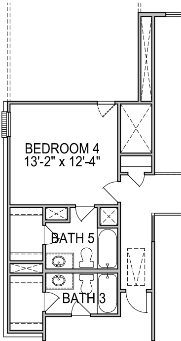
SECOND FLOOR PLAN OPT. #0567 BATH 5
